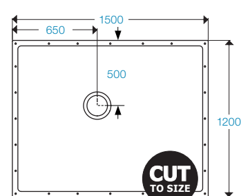
SHOWERDEC® 1500x1200
