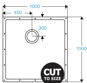
SHOWERDEC® 1000x1000
