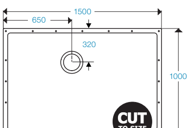
SHOWERDEC® 1500x1000
