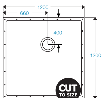
SHOWERDEC® 1200x1200
